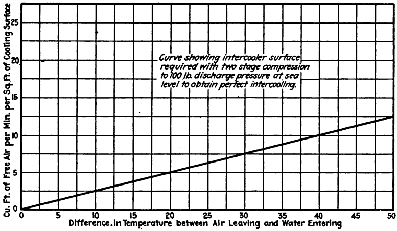
FIG. 61.—Intercooler surface required.
